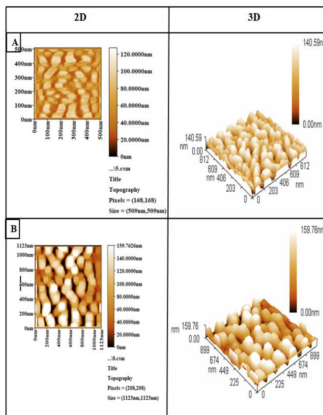
Figure 3: AFM images of the surface roughness coefficients of the filler composite in 2D, 3D (A) At the addition of HAP, (B) At the addition of \text{Fe}_2\text{O}_3 .
